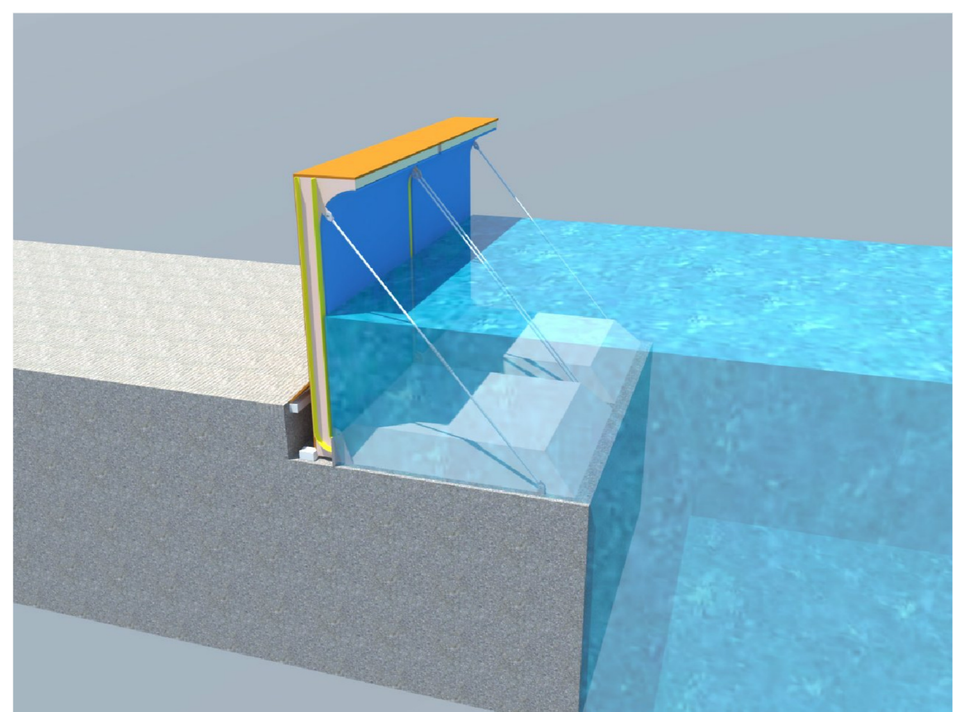
FLOOD PROTECTION Barrier Robust to Applied Loading Adequate Watertightness
